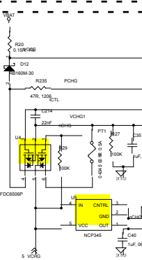
Charging Circuit
