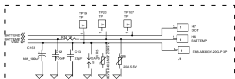
Battery Connector
