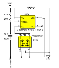
Battery OVP Circuit
