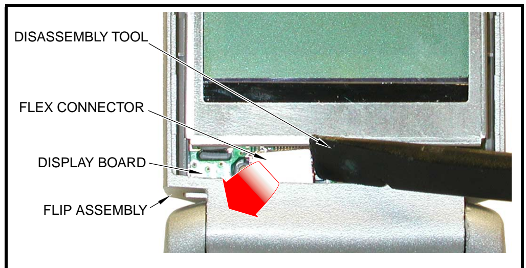
Figure 20. Disconnecting the flex from the display board assembly
