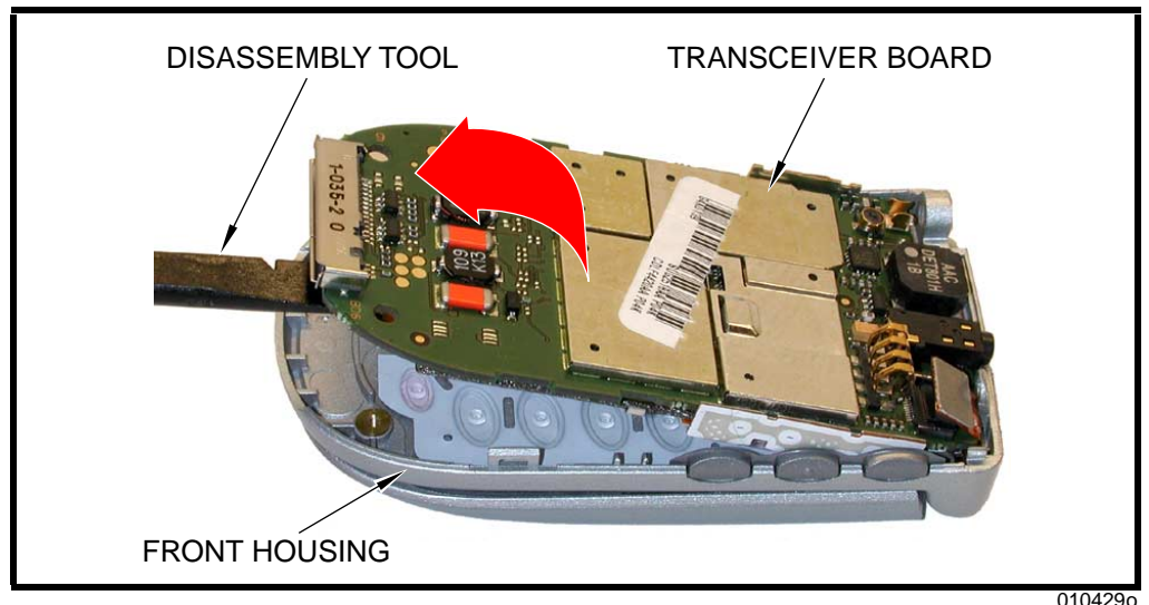
Figure 13. Removing the transceiver board assembly
